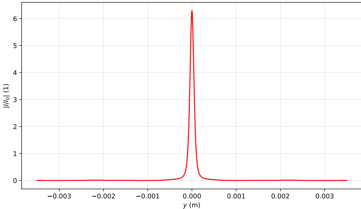
Intensity profile I(x=0, y, z=1.274)/I_0 , P_{in}=5.0P_{cr} , artificial time
